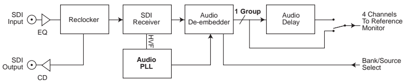
Fig 3-2: RM-HD1 Block Diagram
