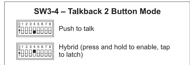
Figure 10. Talkback 2 button mode settings
