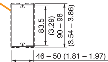
[Dimensions of mounting opening]
