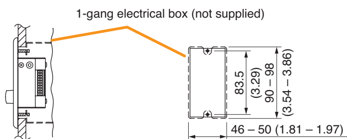
[Figure when mounted]
