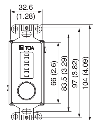
[Front View without panel]
