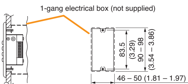
[Figure when mounted]
