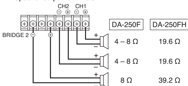
Speaker output terminals
