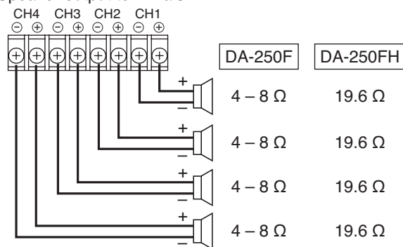
Speaker output terminals
