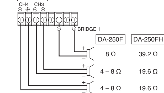
Speaker output terminals
