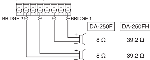
Speaker output terminals
