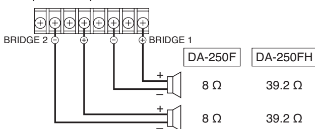
Speaker output terminals
