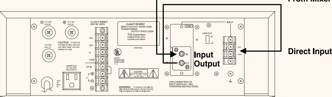
Figure 4 - E Module Connection in P-900MK2
