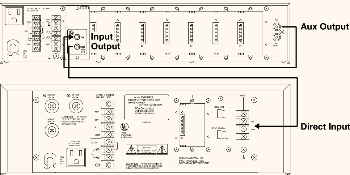
Figure 3 - E Module Connection in M-900MK2 and P-924MK2
