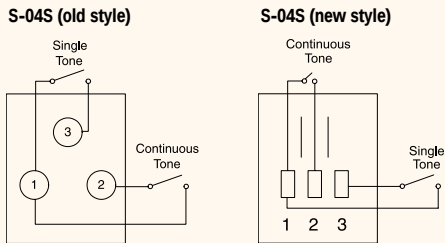
CONNECTOR DIAGRAM
