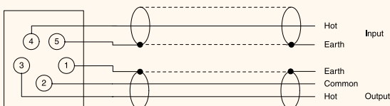
T-02S (Balanced/Unbalanced Output)
