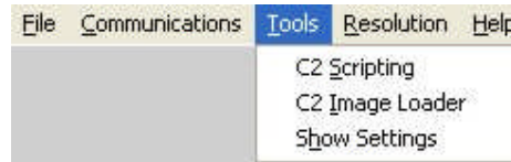
Figure 8 Tools menu
