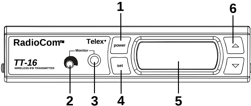
Figure 4a Operating Features TT-16 Front Panel
