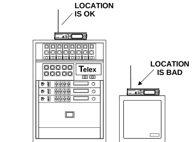
Figure 14 Transmitter Antenna Placement
