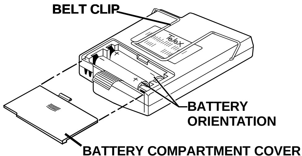
Figure 9 Battery Installation - TR-16
