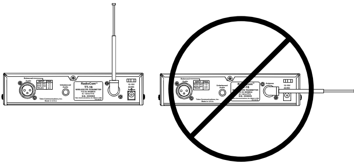
Figure 10 Antenna Alignment Good and Bad
