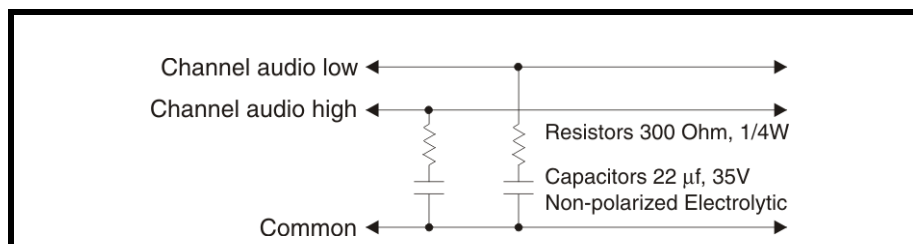
FIGURE 7. Audiocom mode line termination for dry-line operation. (One required for each channel). The termination is available via P/N 9020-7550-000.
