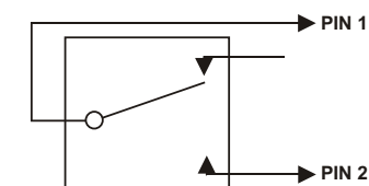
Figure 24 Relay Output Schematic
