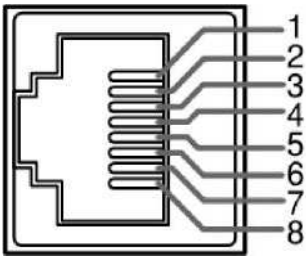
Figure 1–9 RJ45 Connector Pin Map
