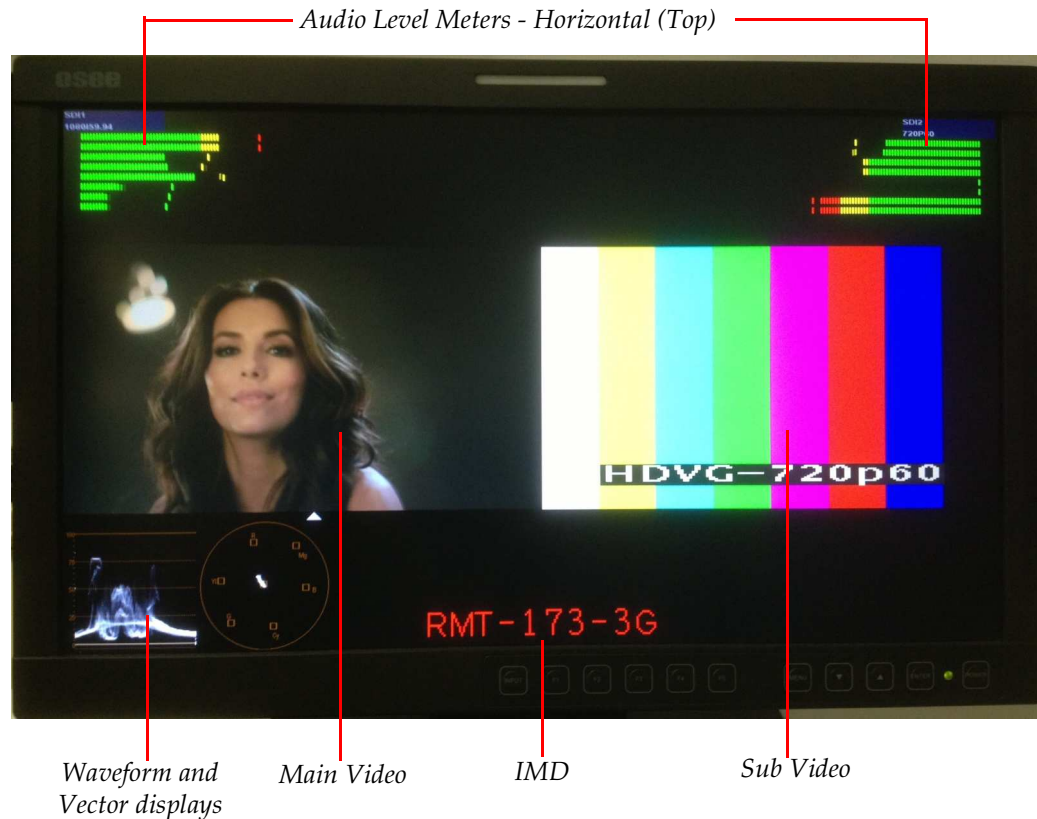
Figure 1-4 RMT-173 PBP Layout
