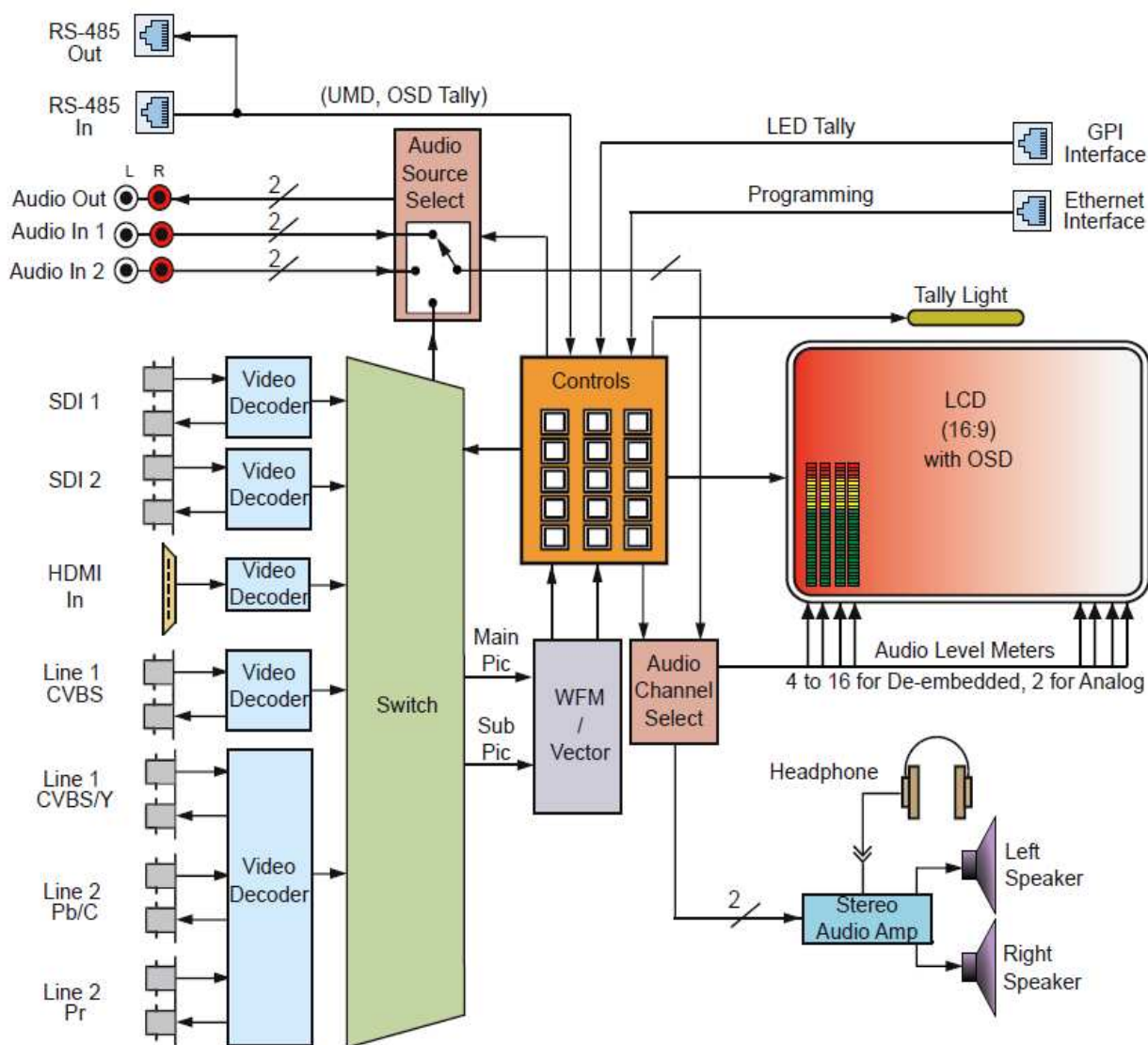
Figure 1-10 RMT-173 Block Diagram
