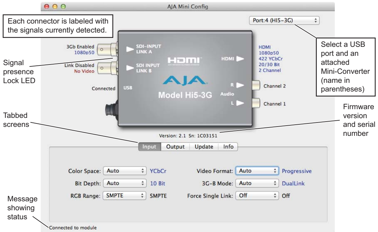
Figure 7. MiniConfig Input Screen
