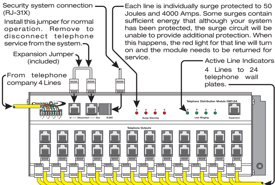
Telephone Distribution Module DMT-24
