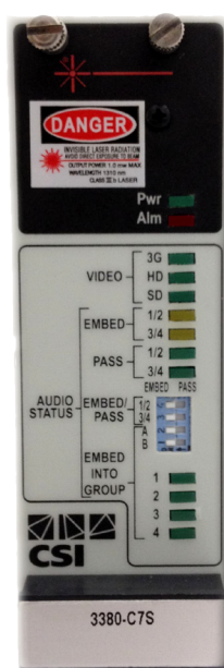
Transmitter Card
