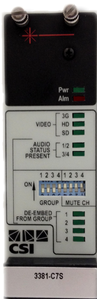
Receiver Card
