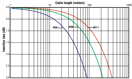
Insertion loss of 4S series speaker cable
