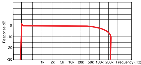
GS-6 Frequency Characteristics (100m, 100Ω > 1MΩ load)
