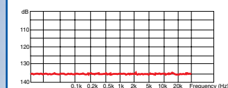
L-4E4-4AT Crosstalk Characteristics (100m)
