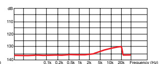
L-4E3-P Crosstalk Characteristics (100m)
