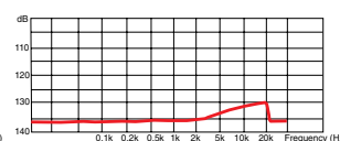
L-4E3-P Crosstalk Characteristics (100m)
