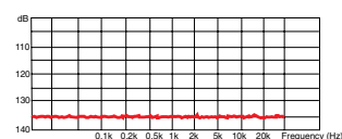
L-4E4-4AT Crosstalk Characteristics (100m)
