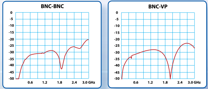
MDVJ-STW Return Loss Chart
