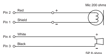
CC-40 WIRING
