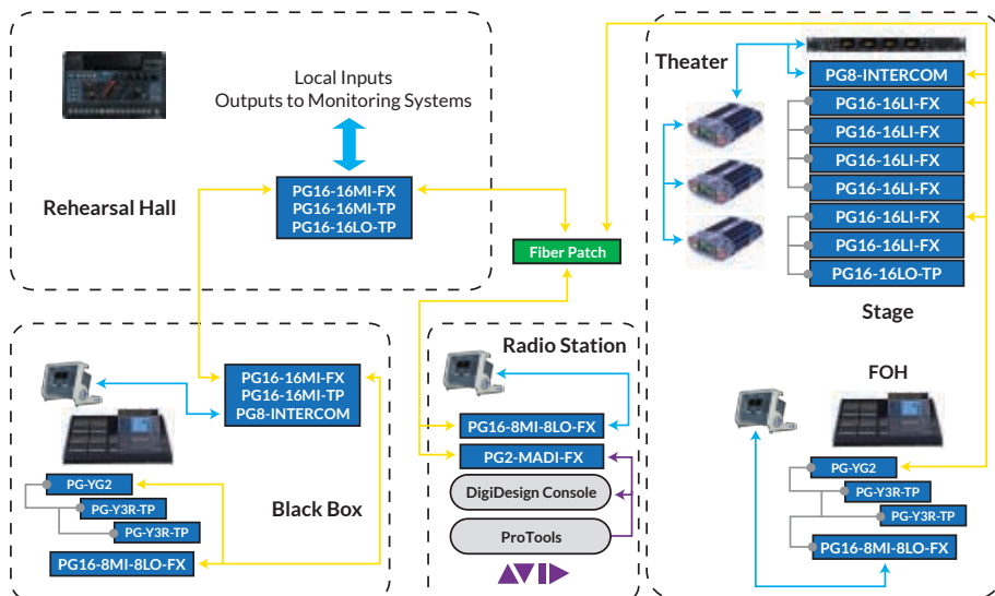
Multiple venues connected to a Studio/Radio Station with HelixNet Intercom over ProGrid
