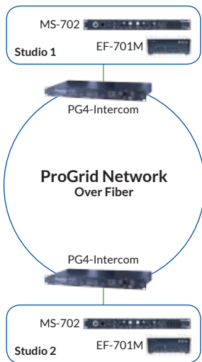
Multiple Encore analog systems connected over ProGrid
