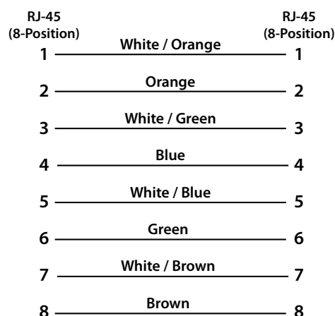
TIA/EIA 568B Straight-Through CAT5e or CAT6
