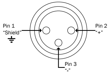
XLR Output Connector Assignment of QTC40
