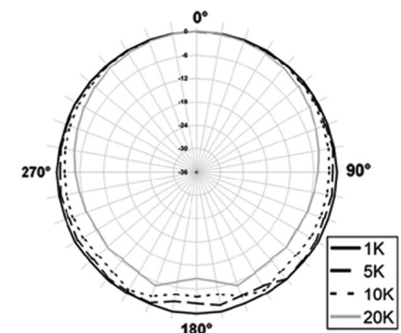
Fig 4. Polar Response (Typical) of TC30
