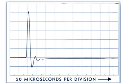
Fig 3. Impulse Response (Typical) of TC30
