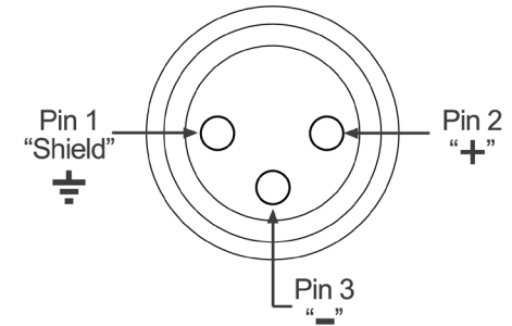
Fig 1. XLR Output Connector Assignment of TC30
