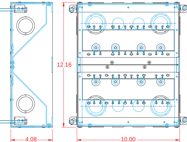
FL-500P-4-B 4" Deep
