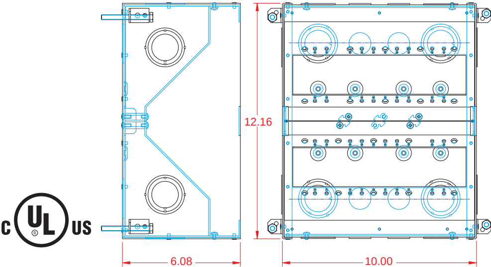
FL-500P-6-B 6" Deep
