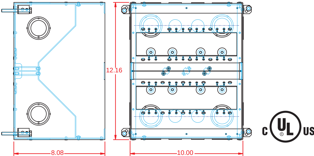
FL-500P-8-B 8" Deep
