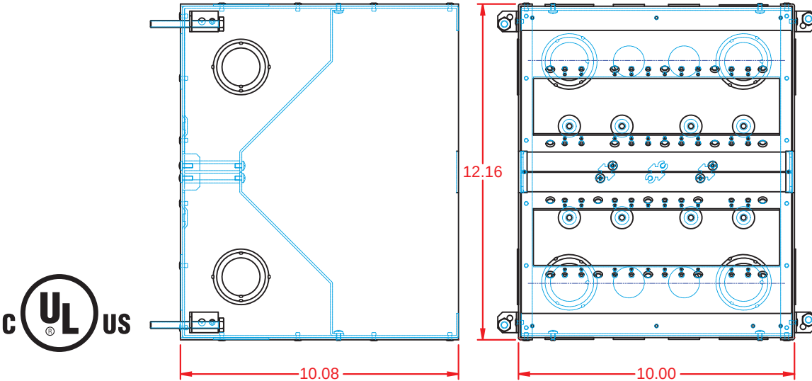
FL-500P-10-B 10" Deep
