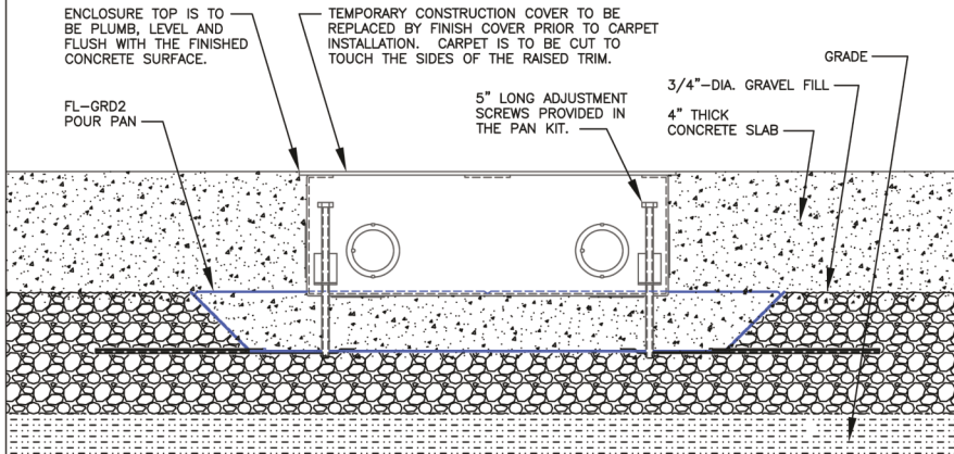
TYPICAL INSTALLATION USING THE FL-GRD4
