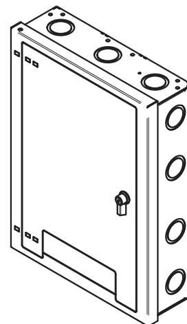
WB-X3-SMCVR SURFACE MOUNTED COVER (SHOWN WITH BACK BOX)
