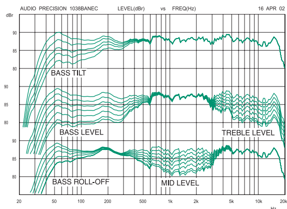
Figure 4: The curves above show the effect of the 'bass', 'mid' and 'treble' level controls, and the 'bass tilt' and 'bass roll-off' controls on the free field response, measured at 2 m.
