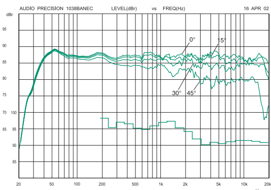
Figure 3: The upper curve group shows the horizontal directivity characteristics of the 1038B in its vertical configuration measured at 2 m. The lower curve is a 1/6 octave power response measure-
