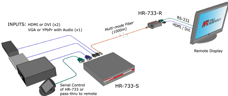
Figure 2 – Block Diagram (HR-731-S only has one HDMI video input)
