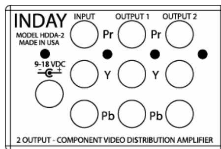
Figure 1 - Connectors
