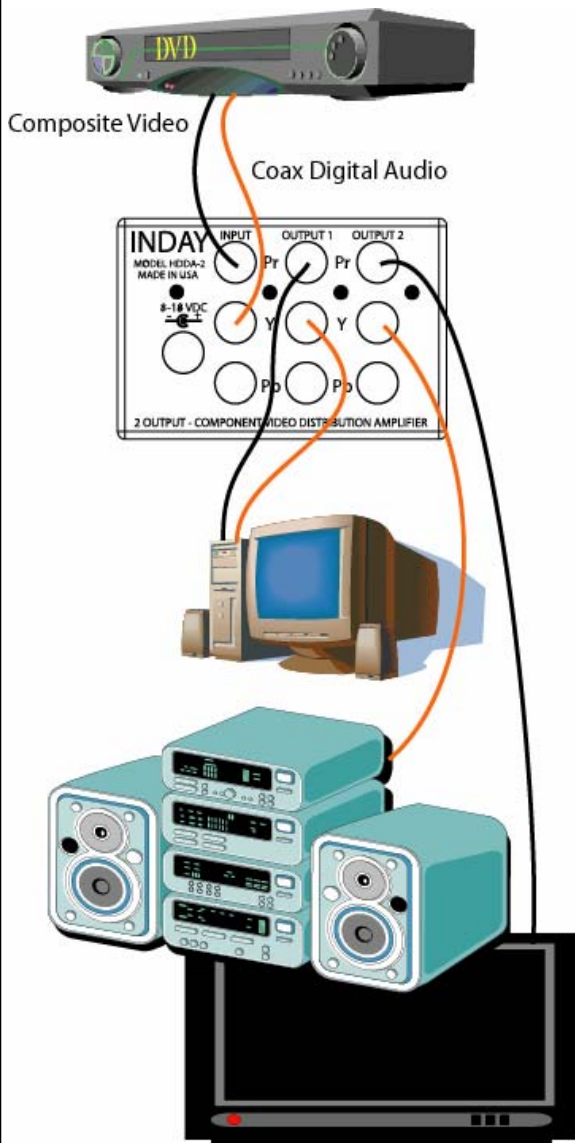
Figure 3 - Home Theater with Video and Digital Audio
