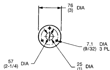
MOUNTING FLANGE DETAIL
