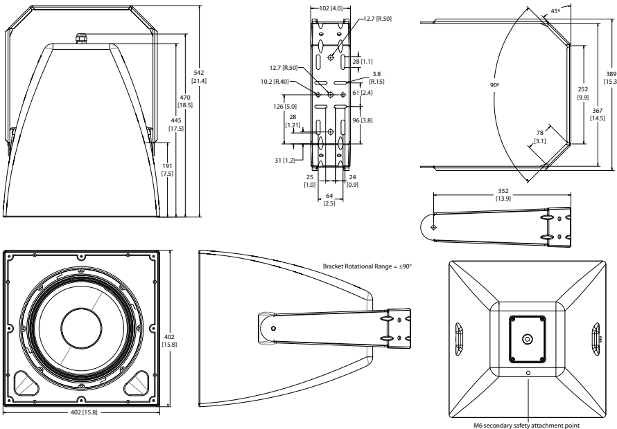
Dimensions in mm (in)
