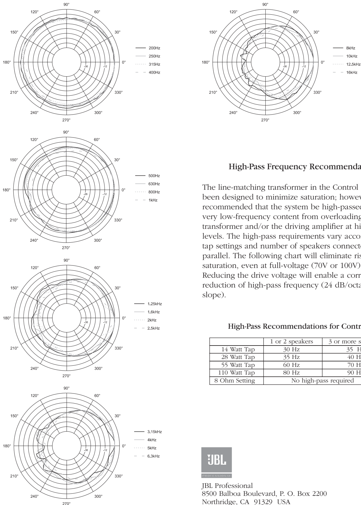
Vertical 1/3 Octave Polars
