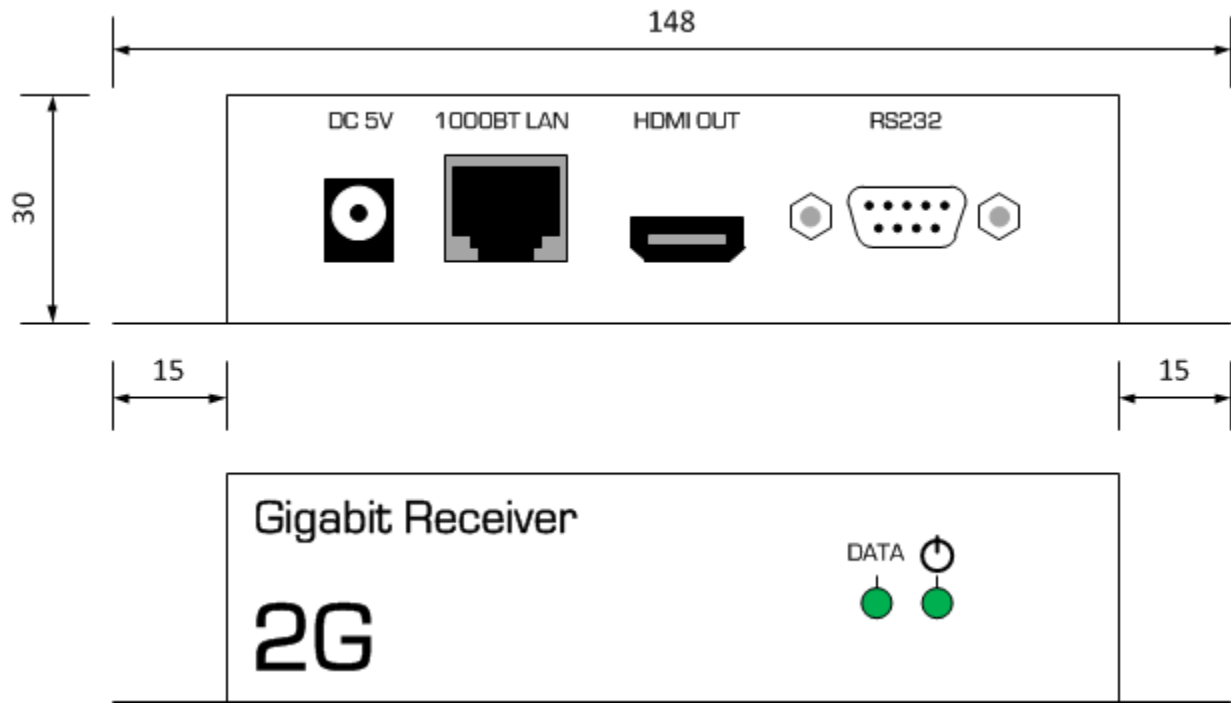
208A Front/Back
