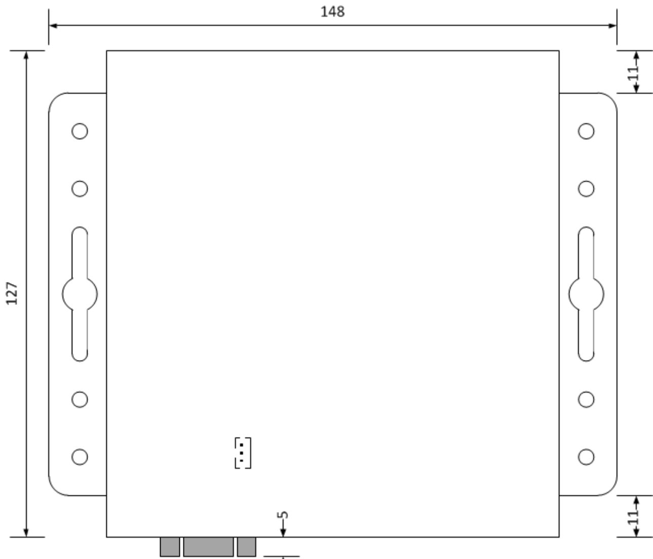
208A Bottom
