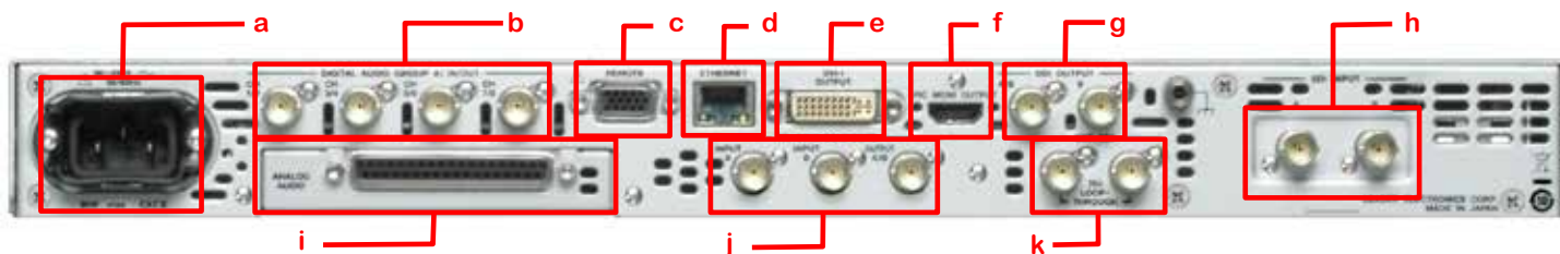
Rear Panel shown with Eye & Jitter Pattern Option, Analog Audio Option, Digital Audio In/Out Option and Composite Inputs Option
