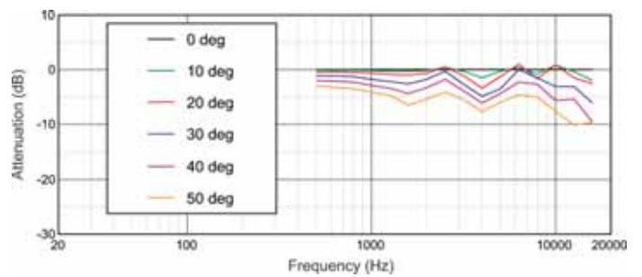
Off-axis, Horizontal
