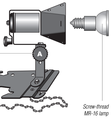
Lock knob for tilting & mount change
