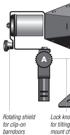
Home-plate mount
