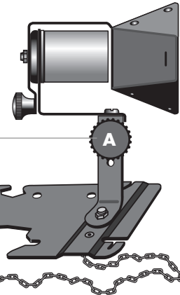
Screw-thread MR-16 lamp
