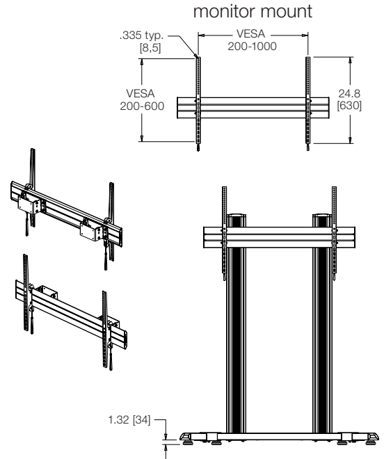
DS-1000SL-AL
