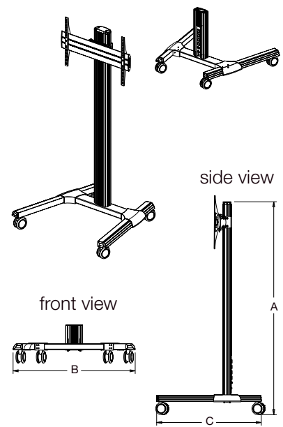
DS-600SC-AL
