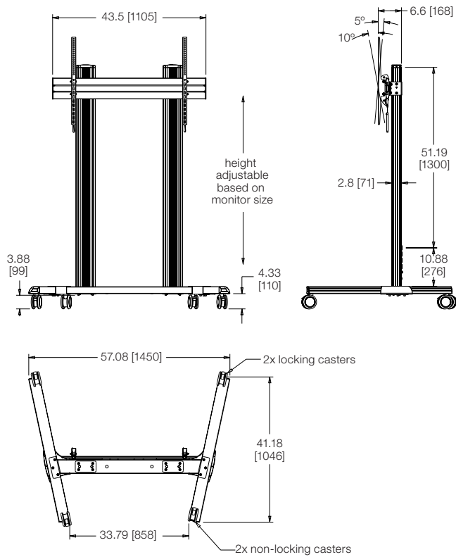
DS-1000SC-AL
