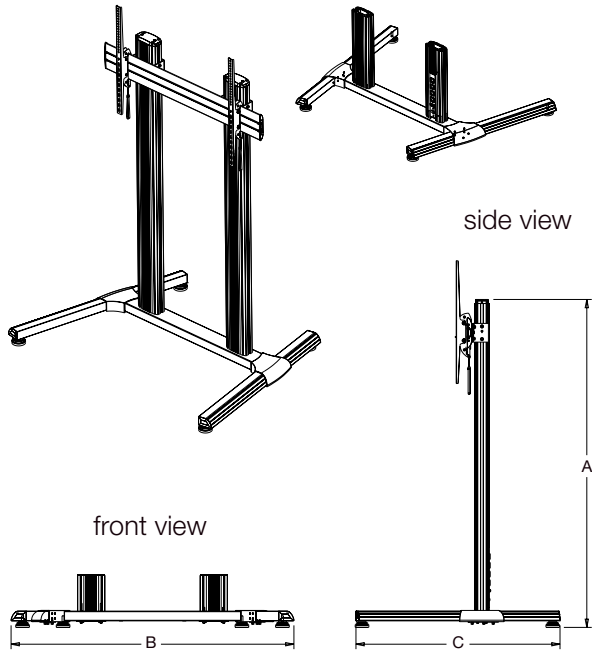
DS-1000SL-AL
