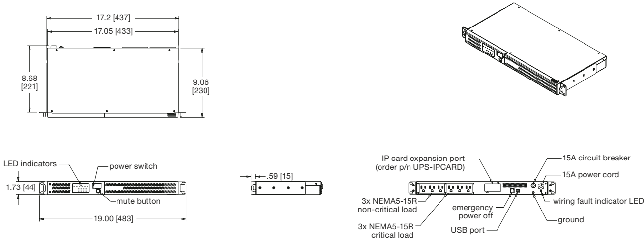
UPS-S500R
