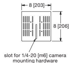
between-display mounting plate included with mount
