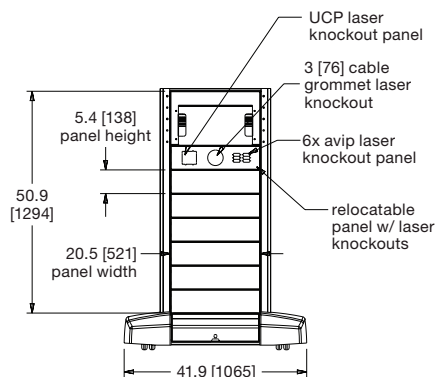
front view monitor and camera mounts removed for clarity
