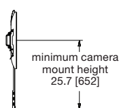
side view bottom camera mount
