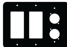
FP-3G-PP2-B 3 Gang Black 2 Decora, 2 XLR
