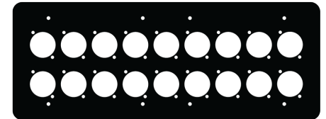
FP-6G-18-B 6 Gang Black 18 XLR
