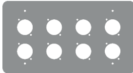
FP-4G-8-S 4 Gang Stainless 8 XLR
