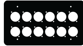
FP-4G-12-B 4 Gang Black 12 XLR
