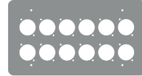
FP-4G-12-S 4 Gang Stainless 12 XLR
