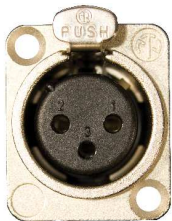
XLRF-D 3-pin XLR female Neutrik® NC3FDL-1
