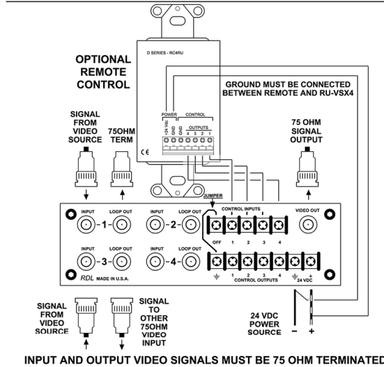
OPTIONAL MOMENTARY REMOTE CONTROL CONNECTIONS SHOWN CONNECTED TO CHANNEL 1 CONTROL MAY USE SWITCH OR OPEN COLLECTOR TRANSISTOR
