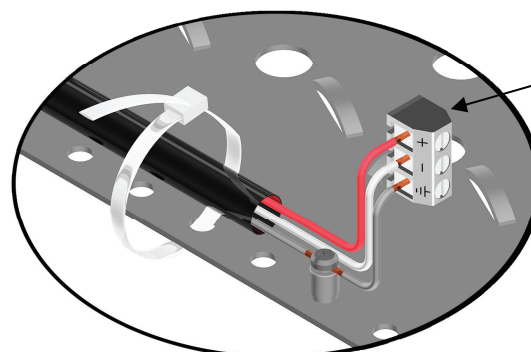
STICK-ON Module Terminal Block
