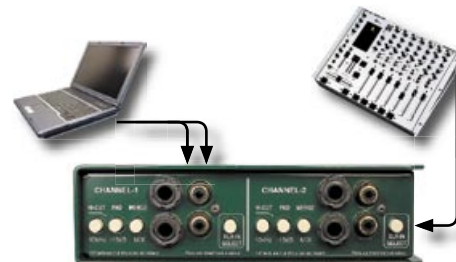
Stereo summed to mono using MERGE function.
