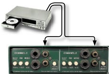
True stereo DI. Connections for 1/4" instruments, -10dB (RCA), and +4dB (XLR) sources.
