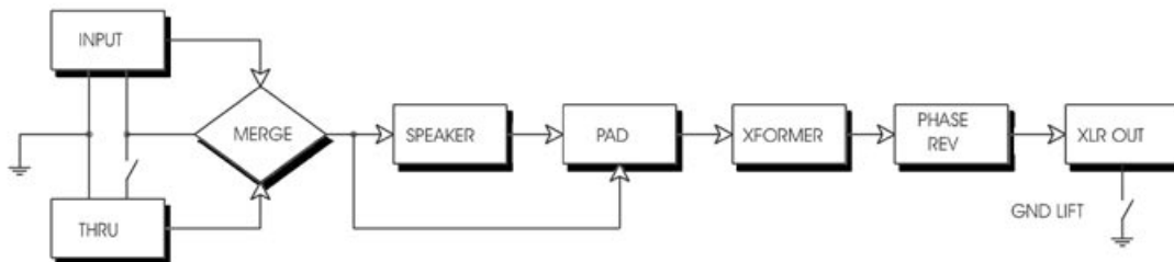
JDI Block Diagram
