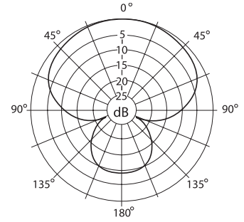
C01U POLAR PATTERN
